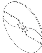
Set Slice Disc of Two Wing Blade Cut size: 1/2/3/4/5/6/8/10mm
