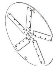
Set Slice Disc of 5-Wing Blade Cut Size: 1/2mm
